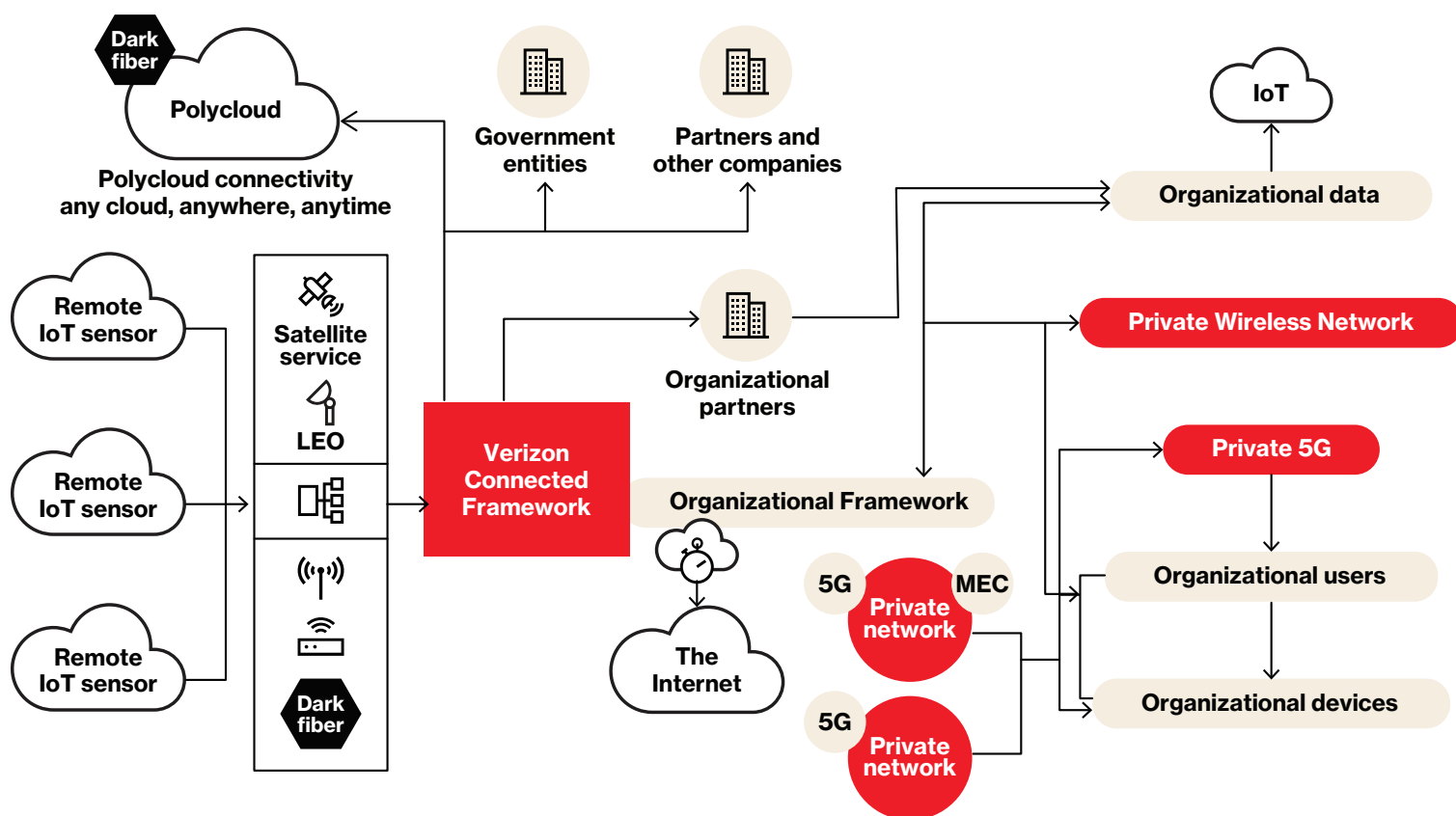
Figure 2. Logical Verizon Framework diagram
